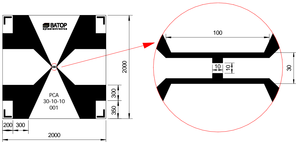
Top view of a photoconductive antenna with l = 30 \mu\text{m} , g = 10 \mu\text{m} , w = 10 \mu\text{m} , No. 001
