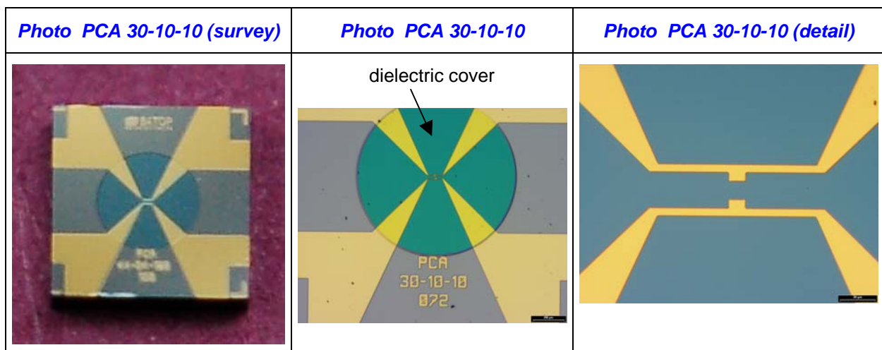
Pictures of a photoconductive antenna with l = 30 \mu\text{m} , g = 10 \mu\text{m} , w = 10 \mu\text{m} , No. 072
